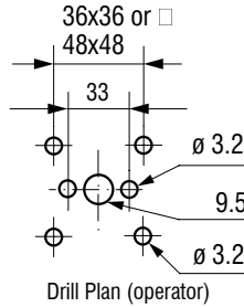
Screw Fixing (RE-40)
