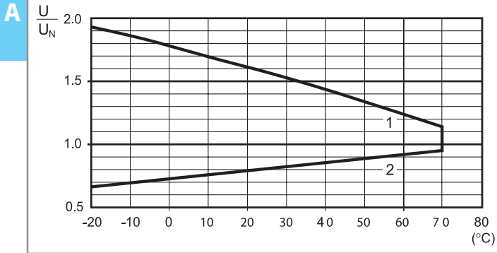
R 60 - DC coil operating range v ambient temperature
