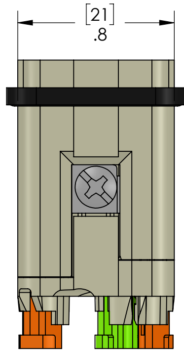
CONTACT SIDE
