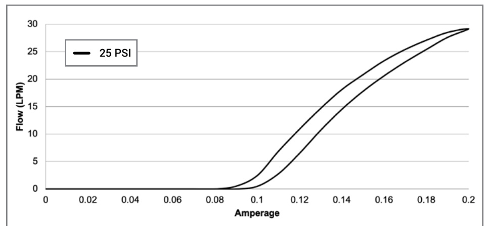
PV10EP2408050 will have precision control but less flow when upstream pressure is lower than 50 PSI. Typical curve with a stabilized upstream pressure of 25 PSI is shown.
