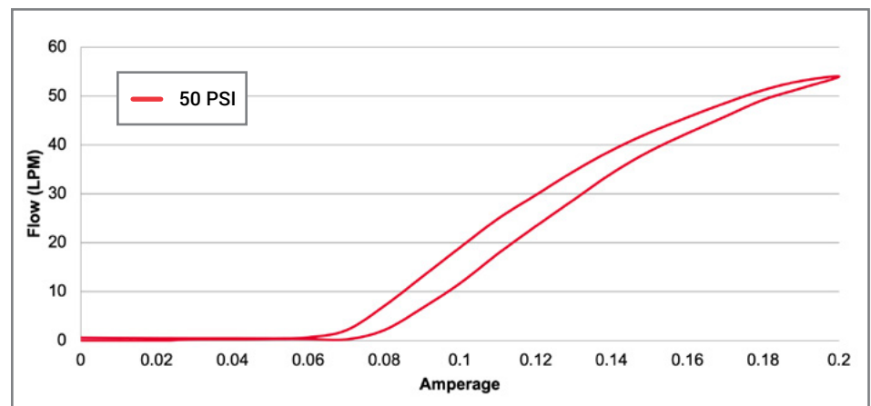
Calibrated with stabilized upstream pressure of 50 PSI to a flow of 50 SLPM @ 200mA.
