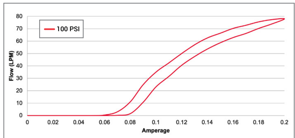
Calibrated with stabilized upstream pressure of 100 PSI to a flow of 75 SLPM @ 200mA.
