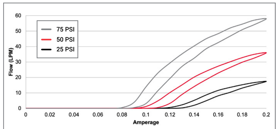
PV10P24080A0 will have precision control but less flow when upstream pressure is lower than 100 PSI. Typical curves with stabilized upstream pressures of 25, 50 and 75 PSI are shown.
