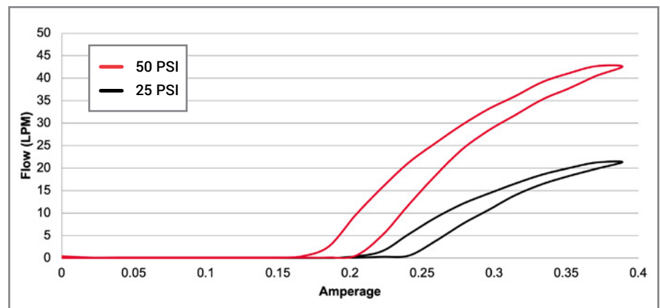
PV10PM1208075 will have precision control but less flow when upstream pressure is lower than 75 PSI. Typical curves with stabilized upstream pressures of 25 and 50 PSI are shown.
