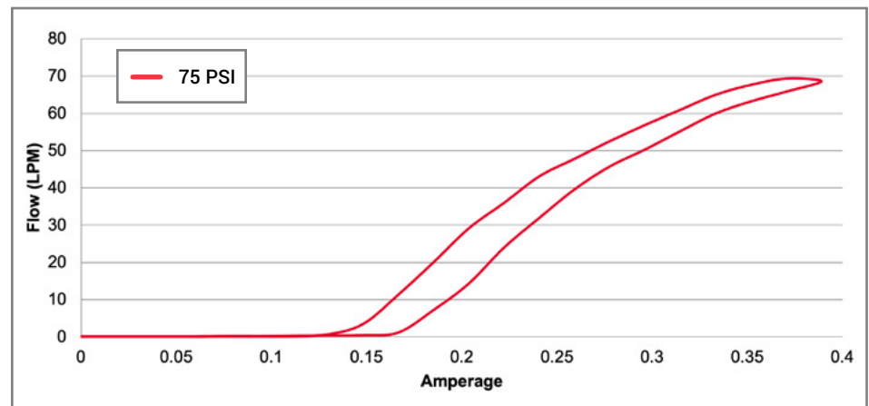
Calibrated with stabilized upstream pressure of 75 PSI to a flow of 65 SLPM @ 400mA.
