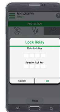
Security setting
