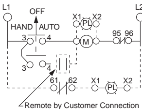
Remote by Customer Connection From top to bottom: Start/Stop, On - Off Selector Switch, HOA Selector Switch
